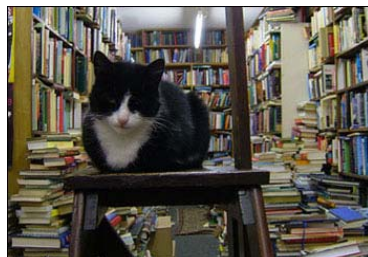
Inventory Management
